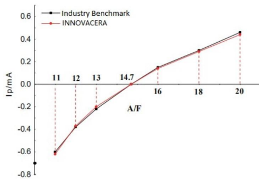
Air-Fuel Ratio Curve
